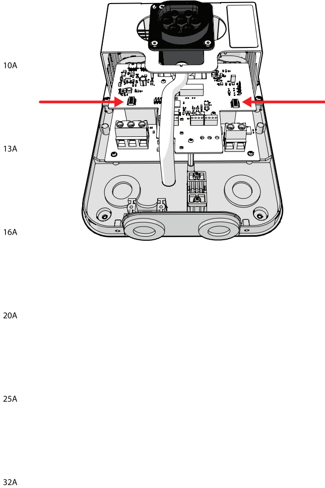
DIP S2
